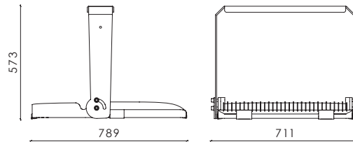
Floodlight console
