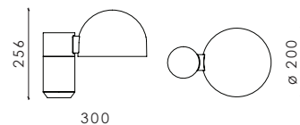
BLACKBIRD MINI POST-TOP (SCREW / TOOL-LESS VERSION) / WITH ZHAGA /
